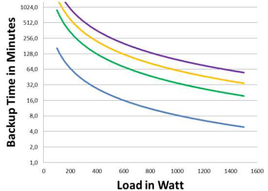
PowerWalker VFI 2000RT LCD
